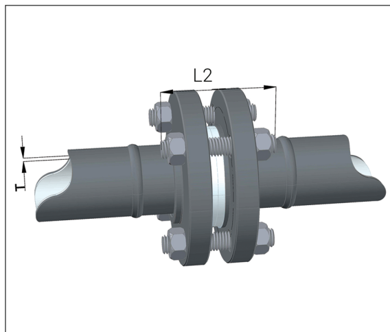
STUB END FLANGES
