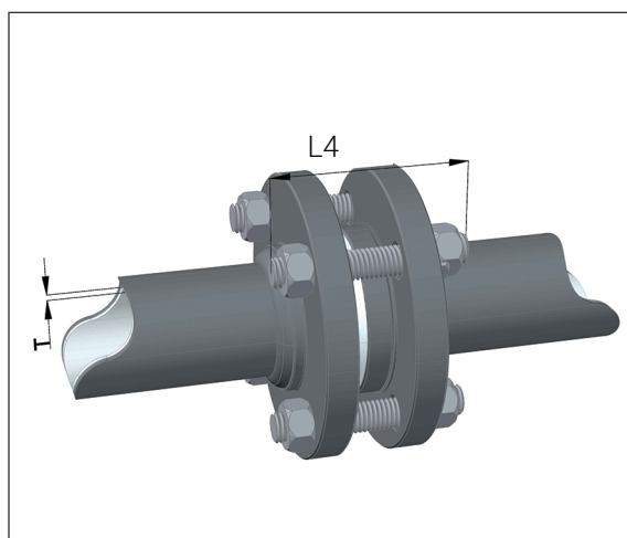
FIXED/ LOOSE COLLAR FLANGES
