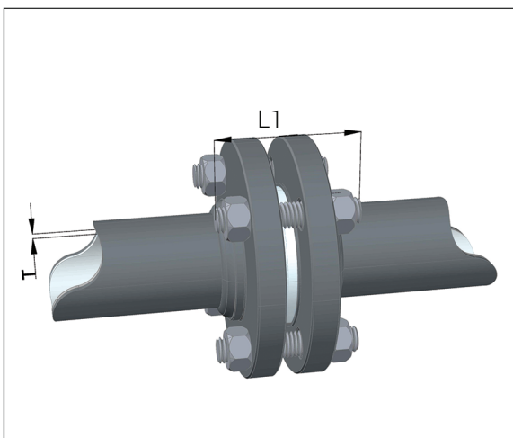
FIXED FLANGES
